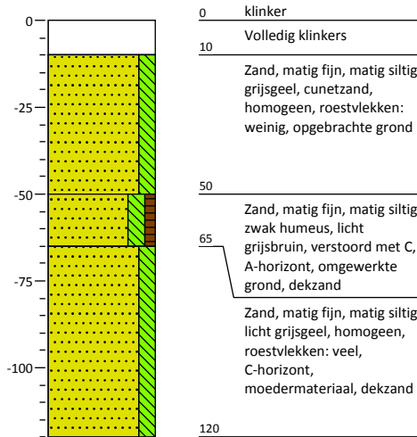
Boring: 002
