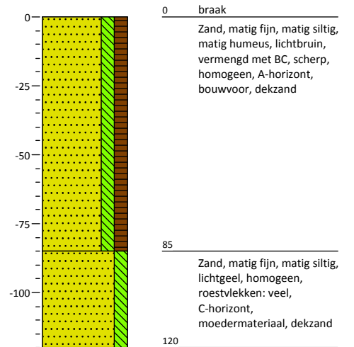
Boring: 006
