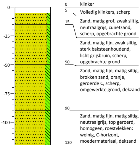
Boring: 004
