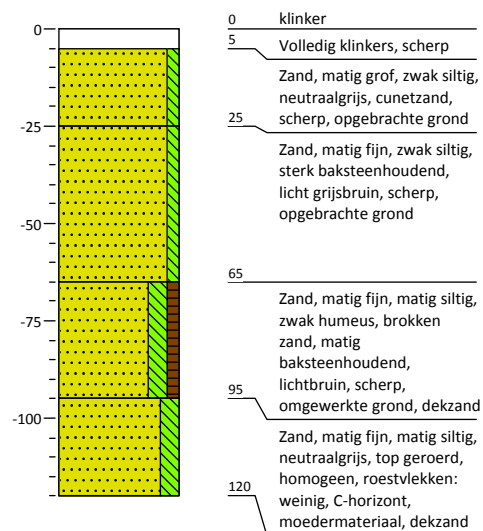
Boring: 018
