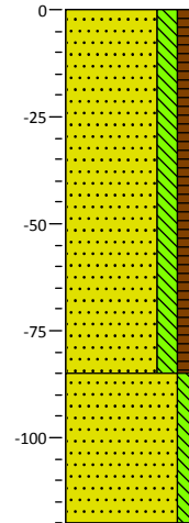
Boring: 009
