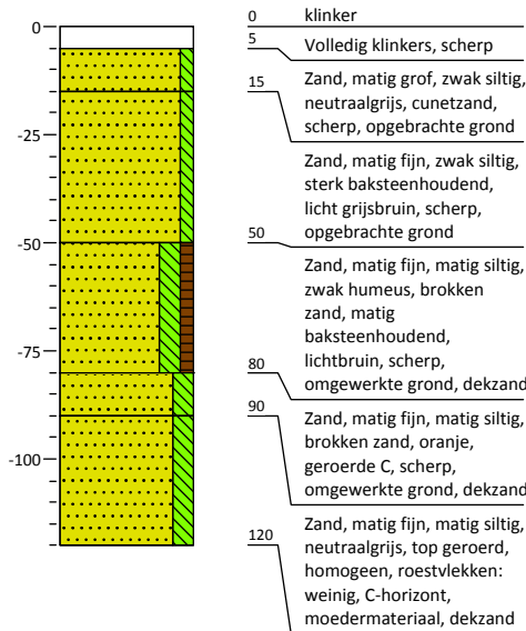
Boring: 005
