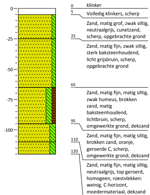
Boring: 015
