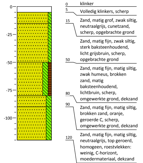
Boring: 003
